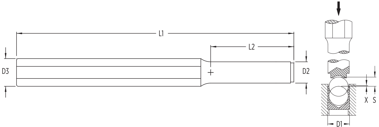
EIS-11, EIS-31 and EIS-33 (Dimensions in mm unless otherwise specified)
